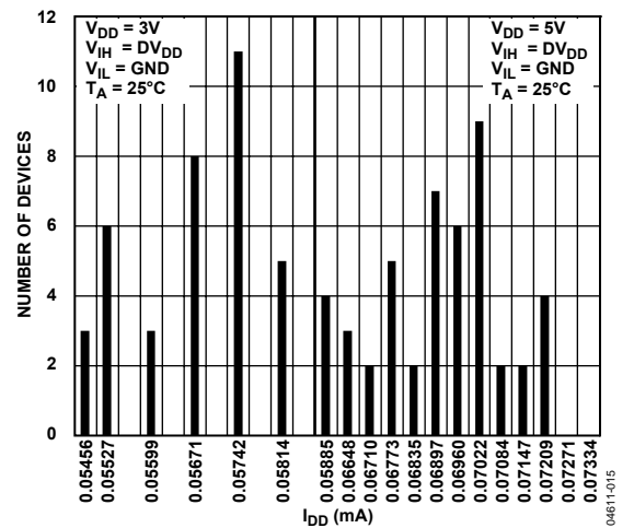
Figure 15. I DD Histogram (3 V/5 V)
