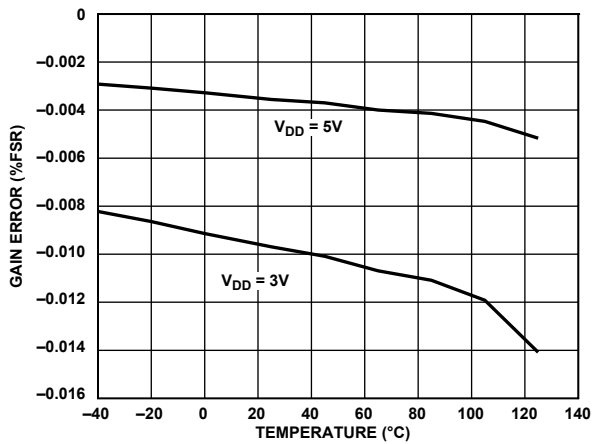
Figure 17. Gain Error vs. Temperature (3 V/5 V)
