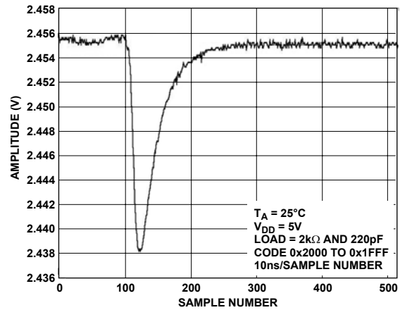
Figure 26. Digital-to-Analog Glitch Energy
