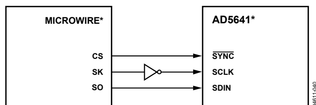
Figure 41. AD5641 to MICROWIRE Interface
