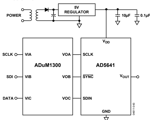
Figure 44. AD5641 with a Galvanically Isolated Interface
