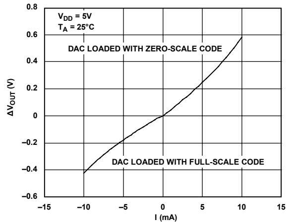
Figure 20. Sink and Source Capability
