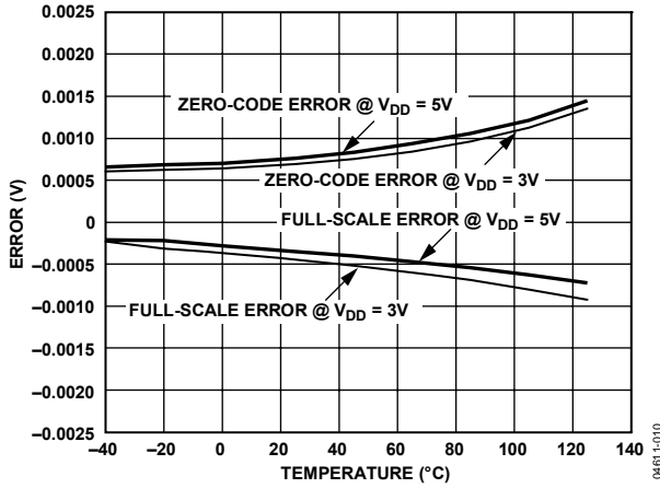
Figure 10. Zero-Code/Full-Scale Error vs. Temperature (3 V/5 V)
