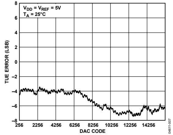
Figure 7. Typical Total Unadjusted Error (TUE)
