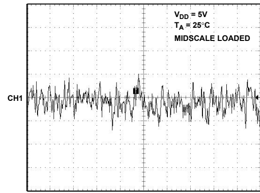
Figure 27. 1/f Noise, 0.1 Hz to 10 Hz Bandwidth
