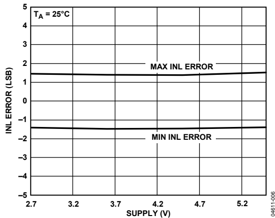
Figure 6. INL Error vs. Supply at 25°C
