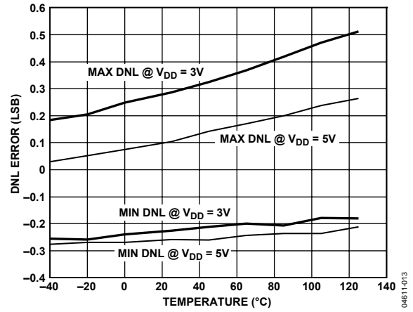
Figure 13. DNL Error vs. Temperature (3 V/5 V)
