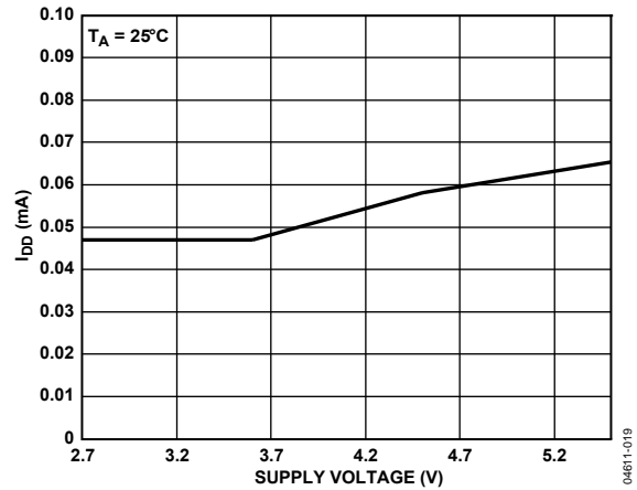
Figure 19. Supply Current vs. Supply Voltage at 25°C
