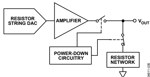
Figure 36. Output Stage During Power-Down
