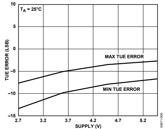
Figure 9. Total Unadjusted Error (TUE) vs. Supply at 25°C
