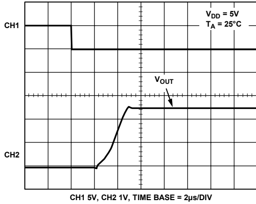
Figure 28. Exiting Power-Down Mode
