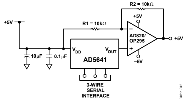
Figure 43. Bipolar Operation with the AD5641
