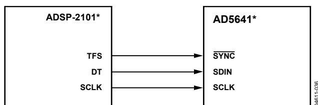
Figure 37. AD5641 to ADSP-2101 Interface
