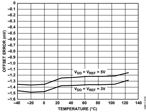
Figure 16. Offset Error vs. Temperature (3 V/5 V Supply)
