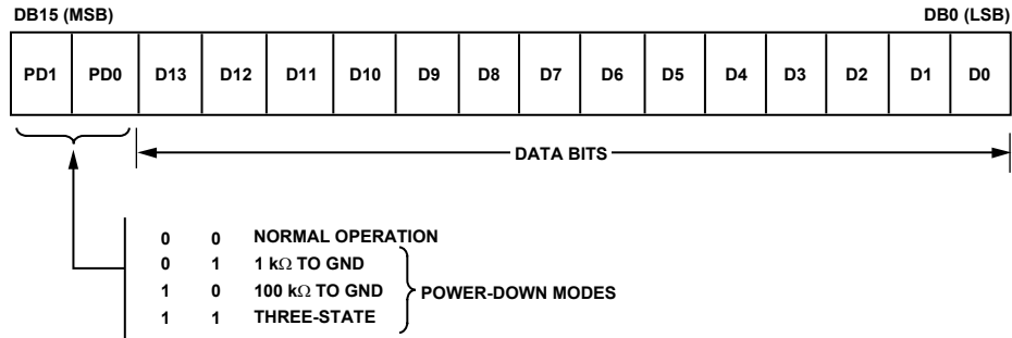
Figure 34. Input Register Contents
