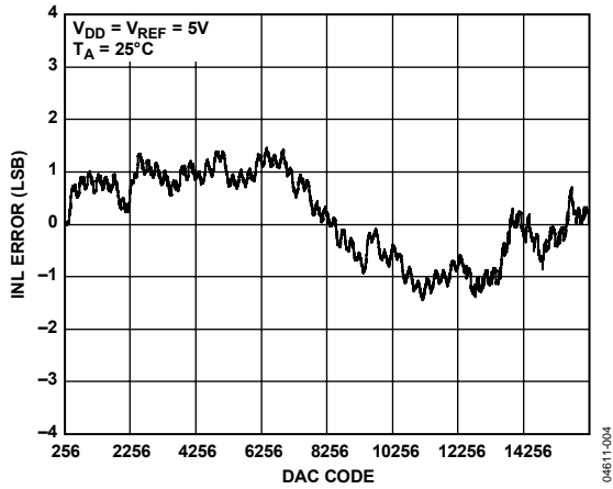
Figure 4. Typical INL
