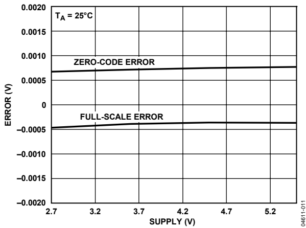
Figure 11. Zero-Code/Full-Scale Error vs. Supply at 25°C
