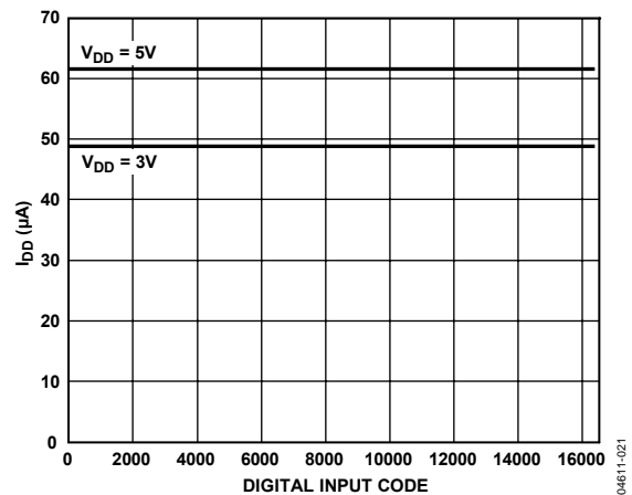
Figure 21. Supply Current vs. Digital Input Code
