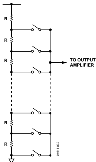
Figure 33. Resistor String Structure
