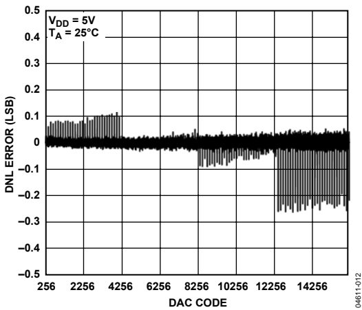
Figure 12. Typical DNL
