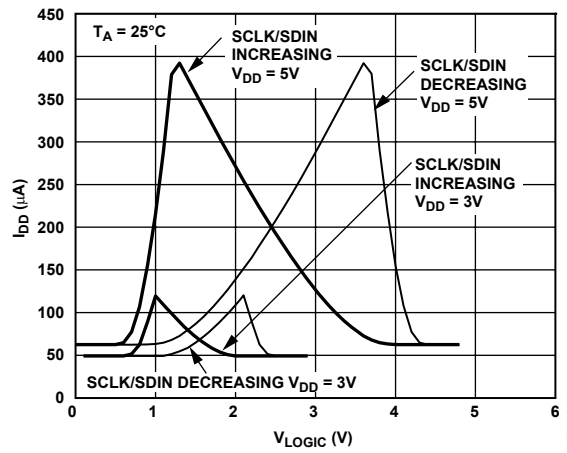
Figure 31. SCLK/SDIN vs. Logic Voltage
