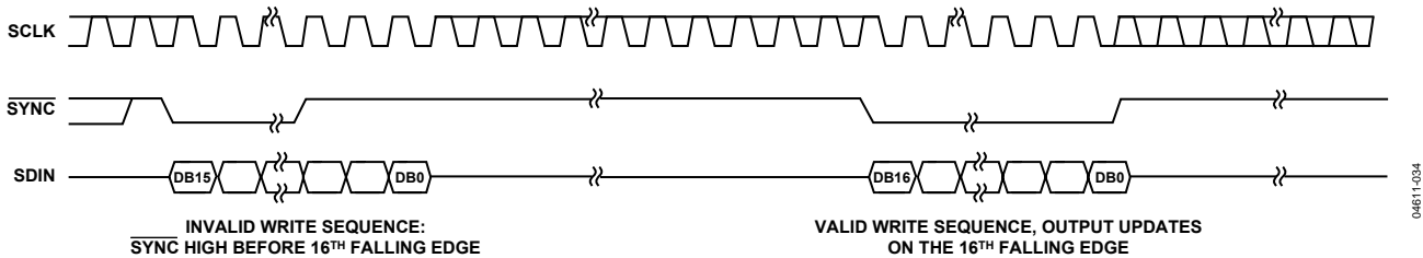
Figure 35. \overline{\text{SYNC}} Interrupt Facility
