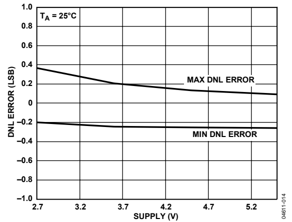
Figure 14. DNL Error vs. Supply at 25°C
