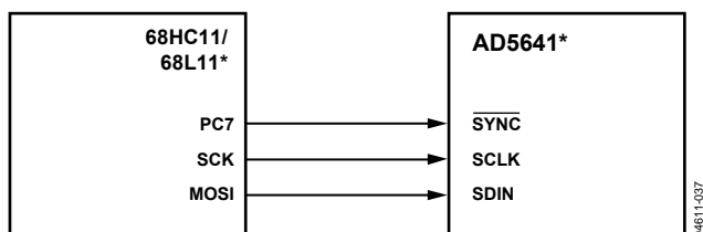
Figure 38. AD5641 to 68HC11/68L11 Interface
