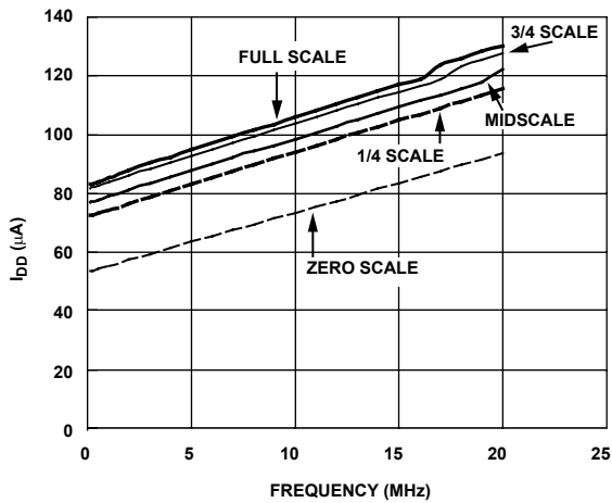
Figure 29. I DD vs. SCLK vs. Code
