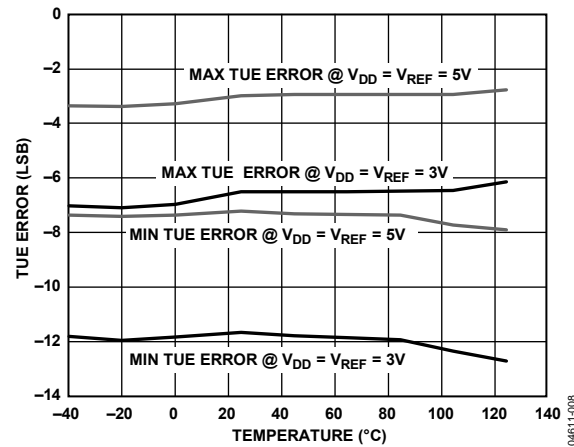
Figure 8. Total Unadjusted Error (TUE) vs. Temperature (3 V/5 V Supply)
