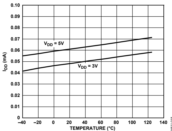
Figure 18. Supply Current vs. Temperature (3 V/5 V Supply)
