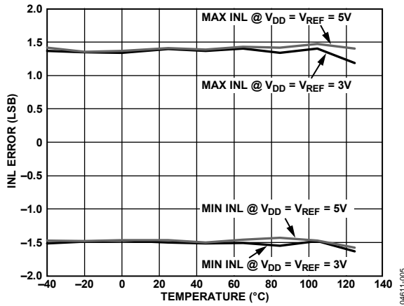
Figure 5. INL Error vs. Temperature (3 V/5 V Supply)
