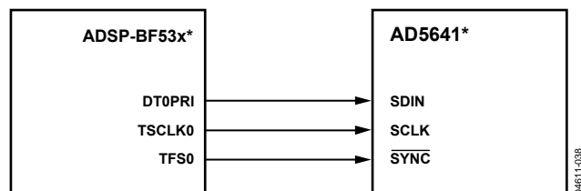
Figure 39. AD5641 to Blackfin ADSP-BF53x Interface
