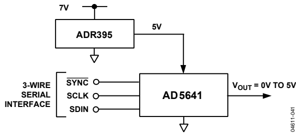
Figure 42. ADR395 as Power Supply to AD5641
