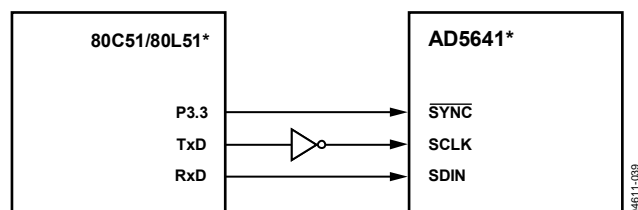
Figure 40. AD5641 to 80C51/80L51 Interface
