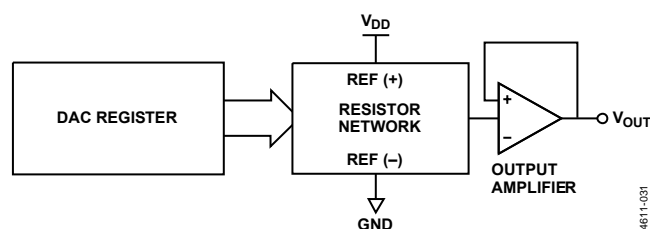
Figure 32. DAC Architecture
