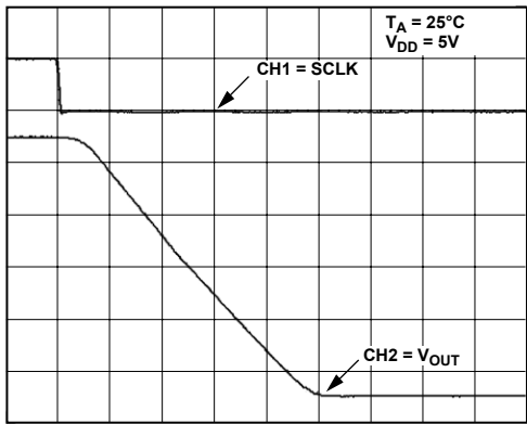
CH1 = 5V/DIV CH2 = 1V/DIV TIME BASE = 2µs/DIV
